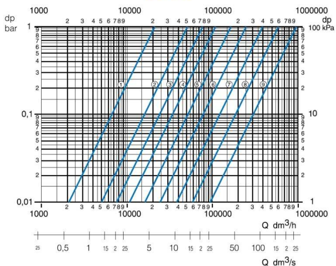
DN250
