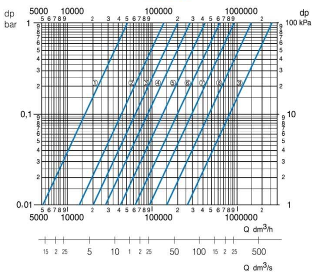
DN250
